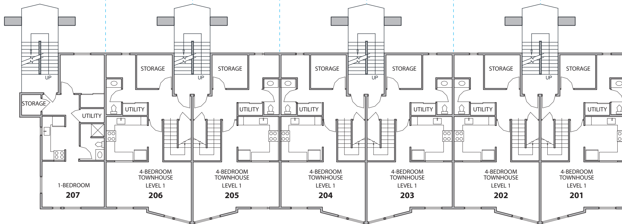
STEVENS COURT - J LEVEL 2 TOWNHOUSE LOWER LEVEL
